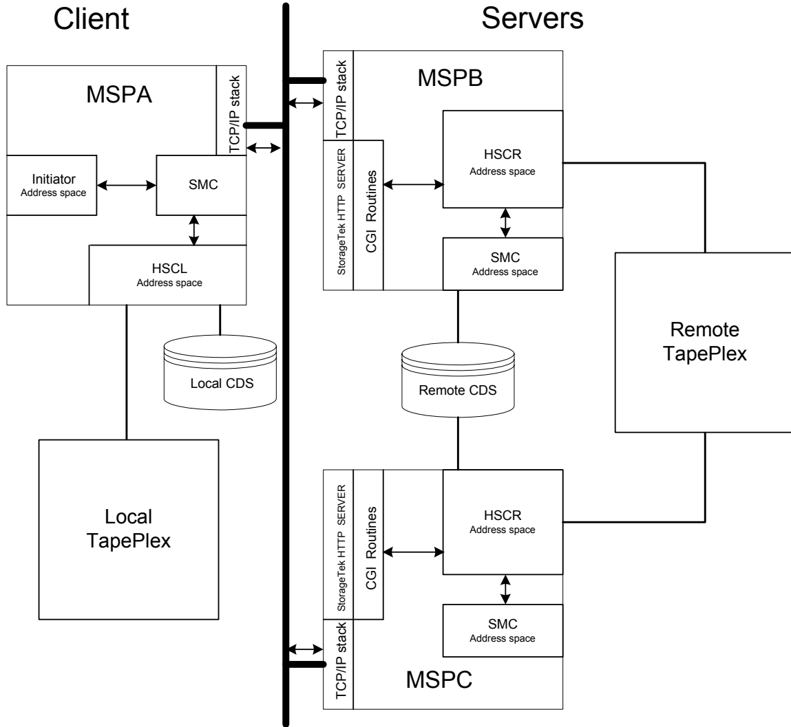
FIGURE 2-6 SMC with Two TapePlexes; One Local and One Remote with Multiple Paths
