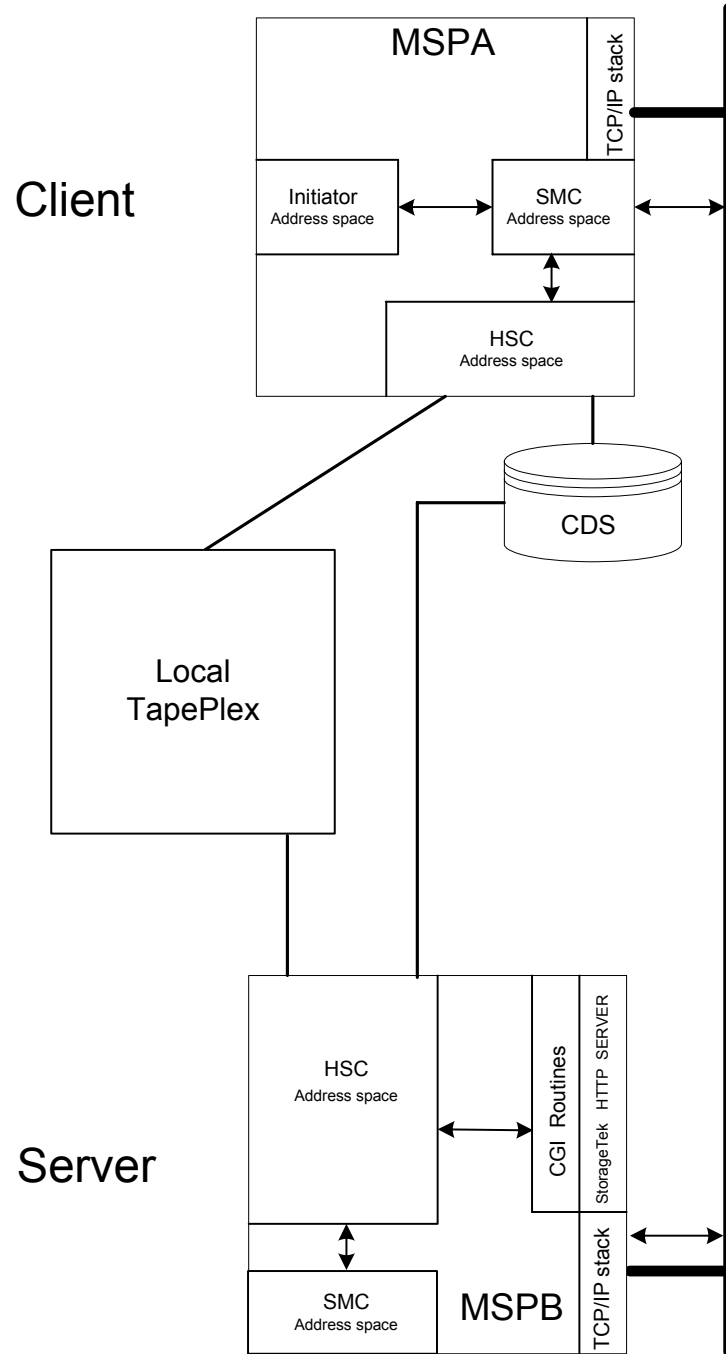
FIGURE 2-3 SMC and a Single HSC TapePlex with One Local and One Remote (alternate) Path
