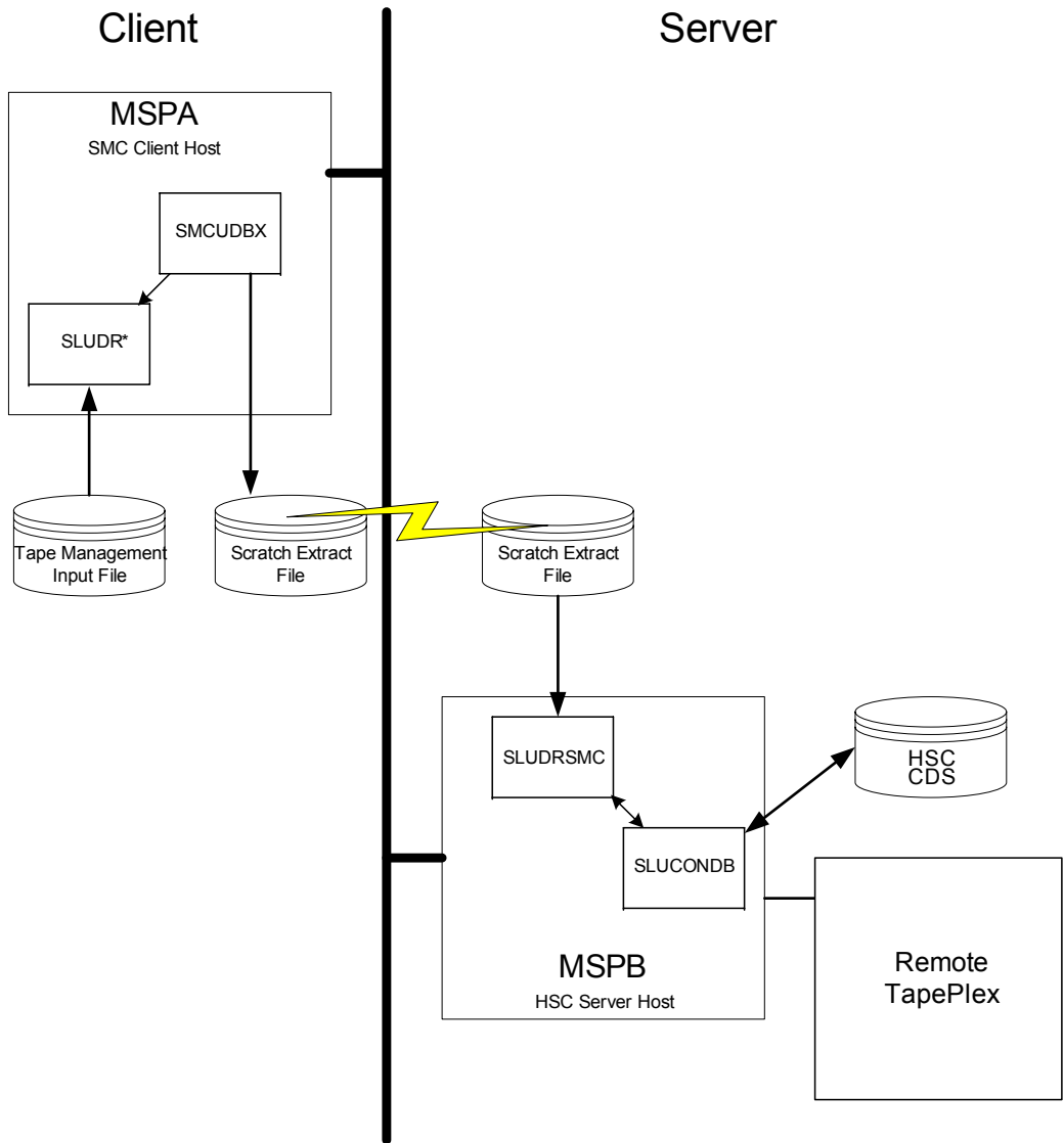
FIGURE 9-1 Scratch Synchronization Between SMC Client host and HSC CDS
